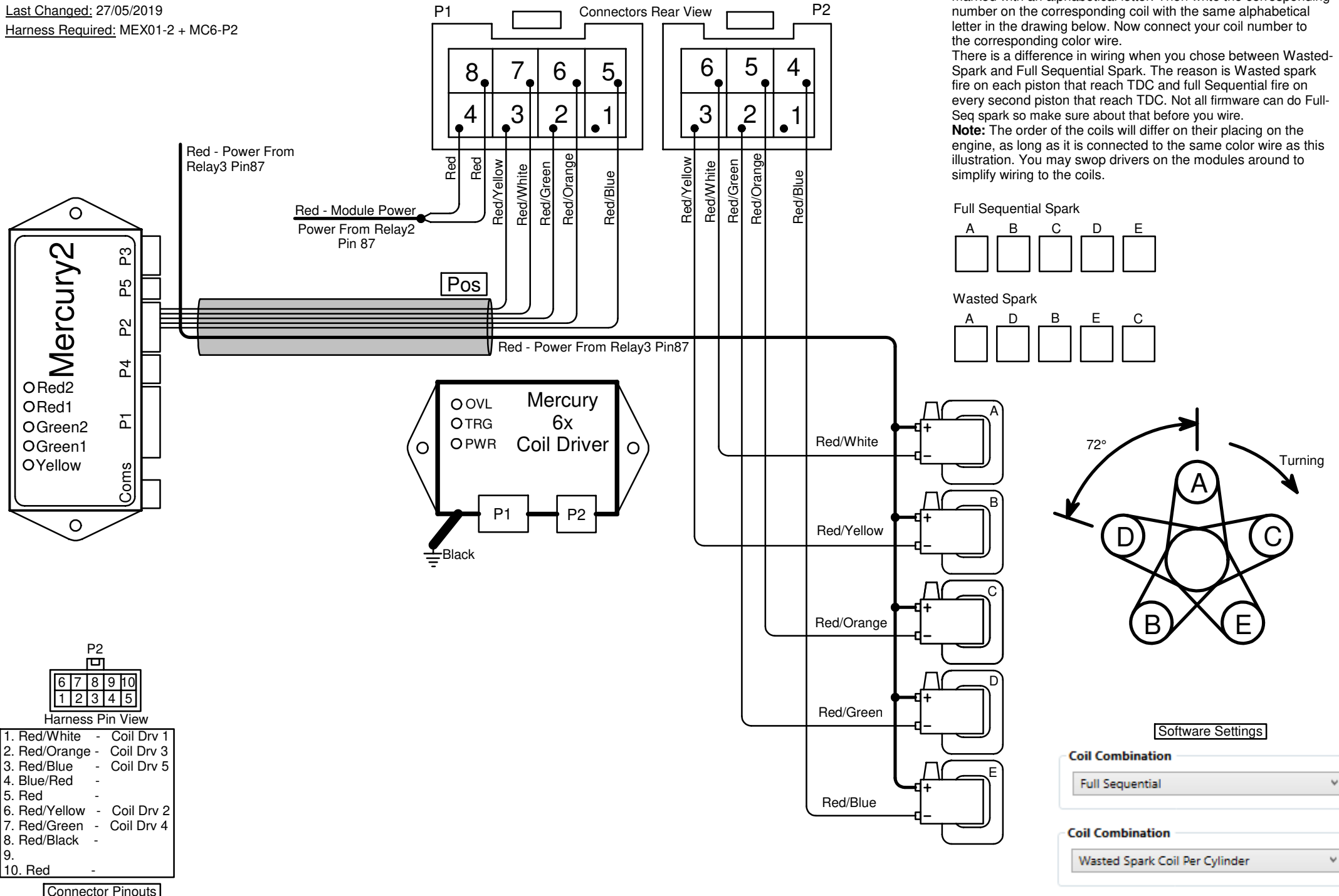
Connector Pinouts
