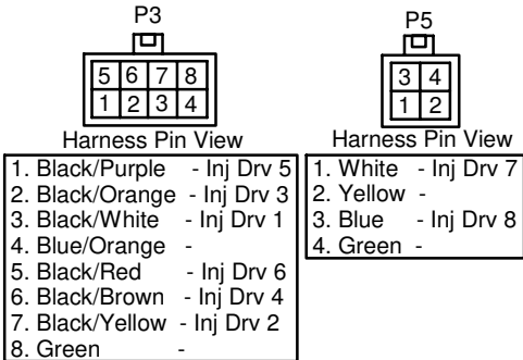
Connector Pinouts
